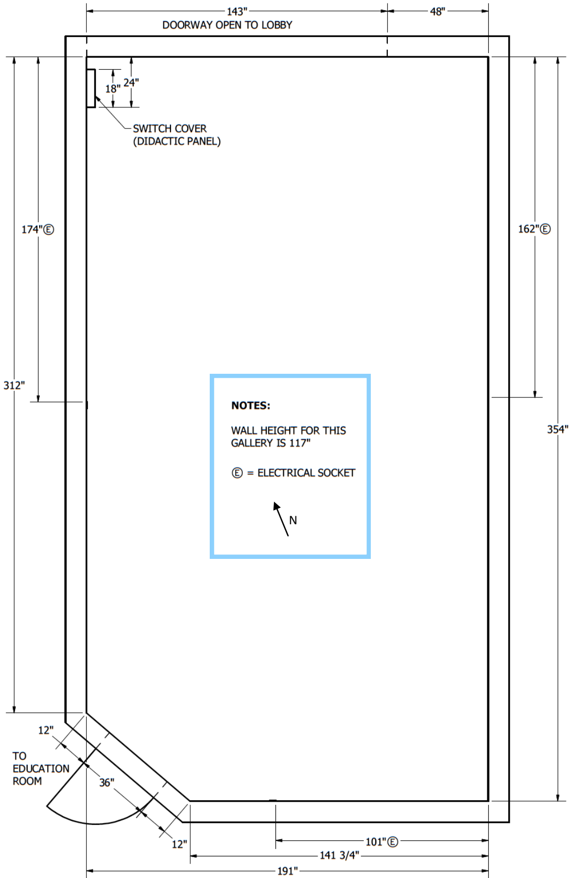
EAGM Gallery 2 floor plan
